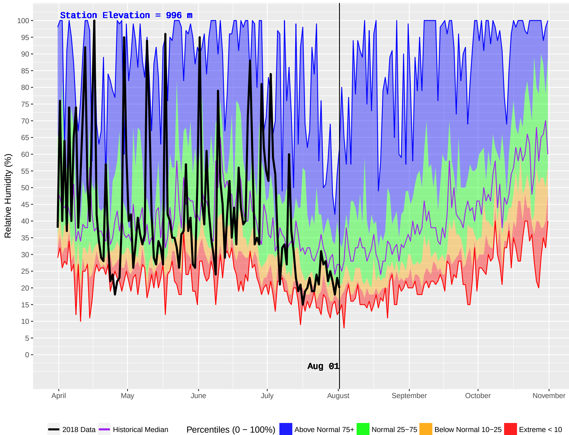
CRANBROOK FS (426) : Historical (2001–2016) and Current (2018) Daily Relative Humidity
